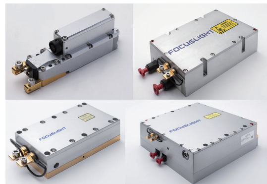
Bar-based fiber coupled modules: LM, FG, ND, MF series
