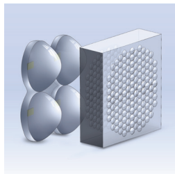
Semi-dynamic system example: MLA with 4 channels, LED, 4 collimators
