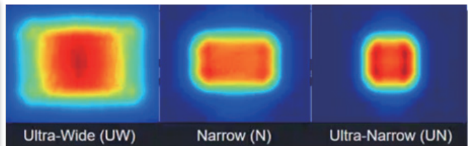
Irregular Micro Lens Arrays (diffusers) for flood illuminators with various FOIs
