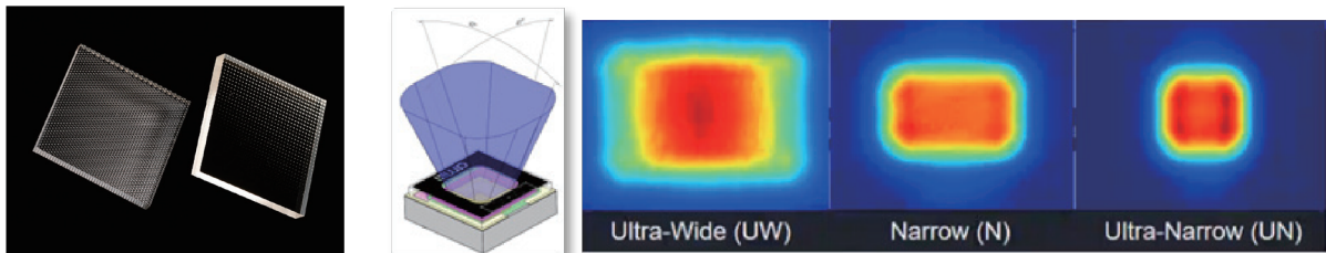
Irregular Micro Lens Arrays (diffusers) for flood illuminators with various FOIs
